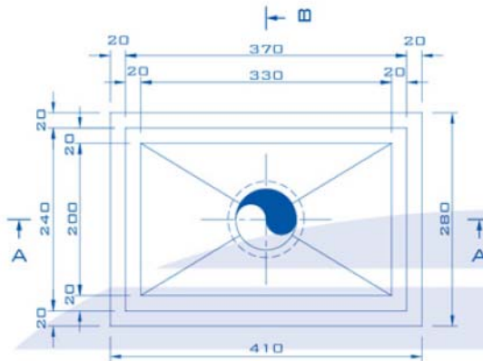
SCUPPER PLAN
