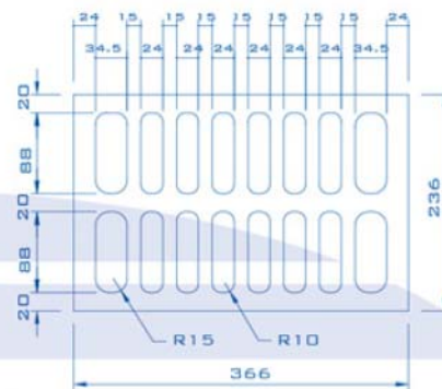
GRATING DETAIL
